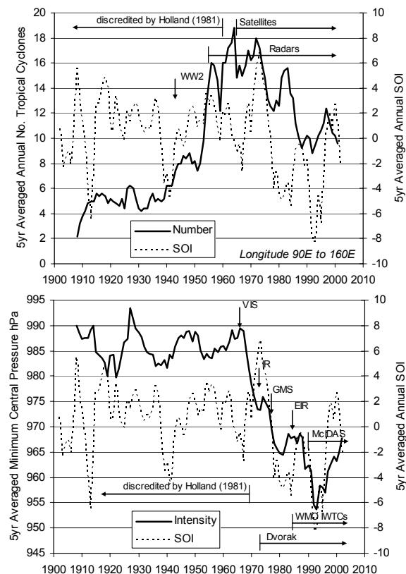
Figure 1 Australian Region best track data example.
